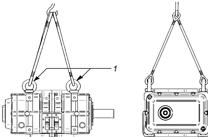
1 Eyebolts
