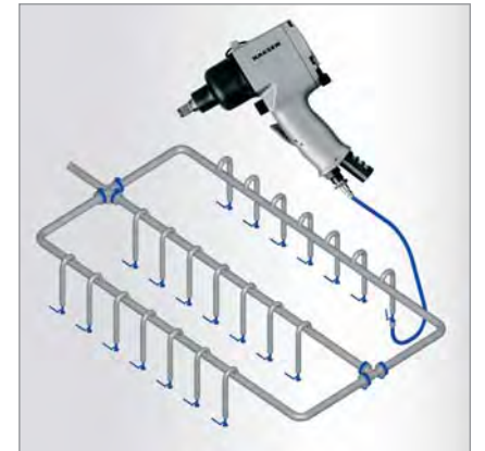
Fig. 4: Leakage measurement of compressed air consumers + air distribution network
