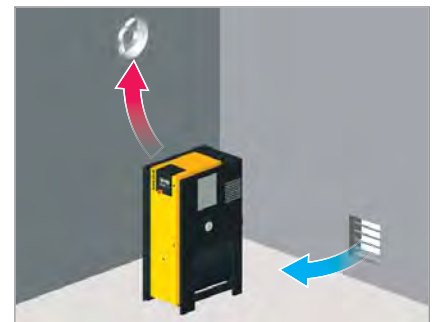
Fig. 2: Forced ventilation with extractor fan for compressors from 5.5 to 11 kW
