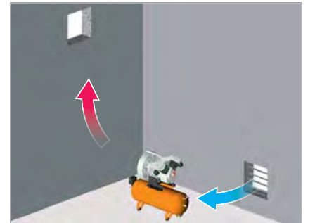
Fig. 1: Natural ventilation for compressors up to 5.5 kW
