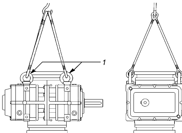
1 Eyebolts
